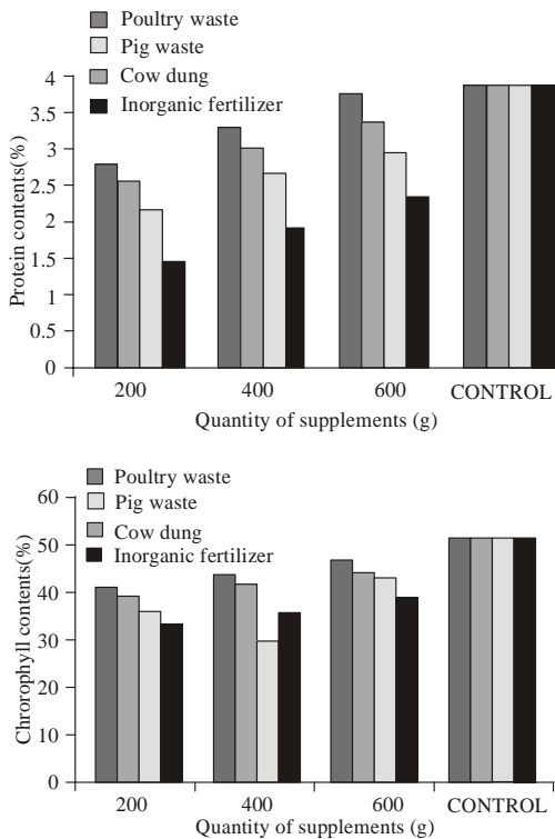
Fig. 1: Protein (A) and chlorophyll (B) content of eggplant in heavy diesel oil polluted soil
