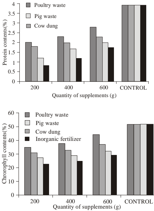
Fig. 1: Protein (A) and chlorophyll (B) content of eggplant in heavy diesel oil polluted soil
