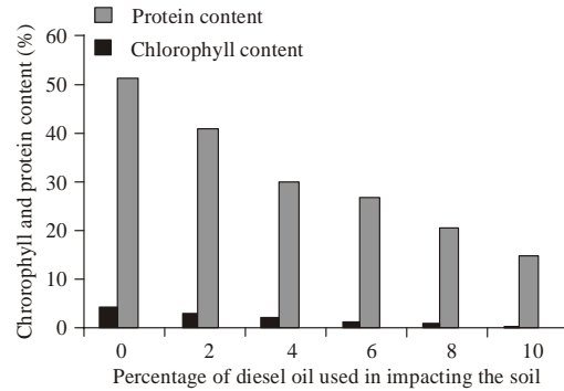
Fig. 3: Protein and chlorophyll contents of eggplant on soil s polluted with different concentration of diesel oil
