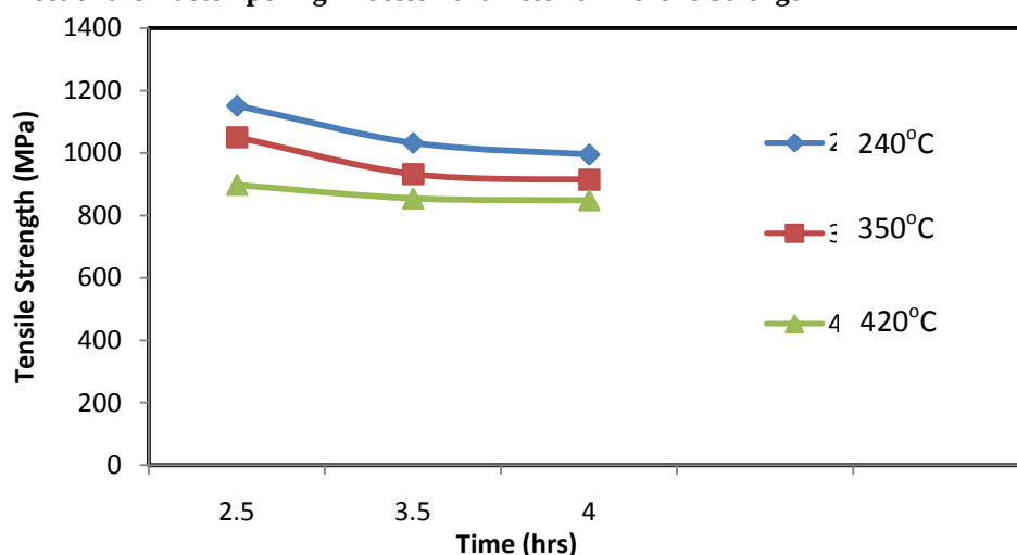
Fig. 3.1: Effect of austempering temperature and time on tensile strength of ADI material
