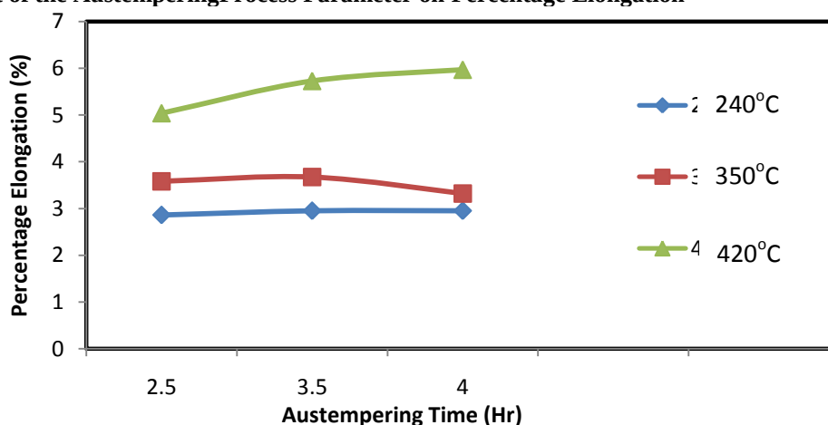
Fig. 3.2: Effect of austempering temperature and time on the percentage elongation of ADI material
