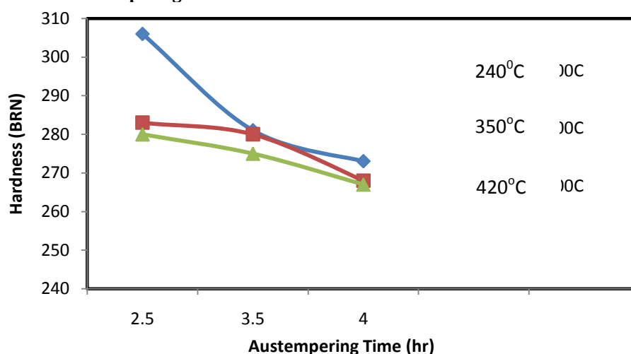
Fig. 3.3: Effect of austempering temperature and time on the hardness of ADI material
