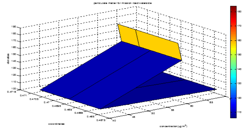
Matlab Surface Plot of PM 10 for Mission Road/Waterside,Onitsha (Rain)
