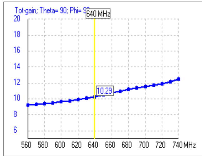
Fig 4. Total Gain vs. Freq.
