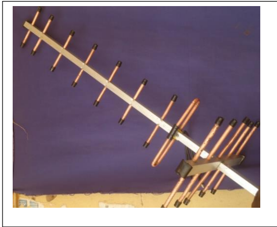
Fig 6. Fabricated antenna
