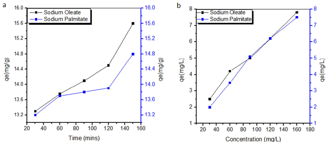
Figure 4. (a) Effect of time on adsorption of soap molecules on natural barite; (b) effect of concentration on adsorption of soap molecules on natural barite.
