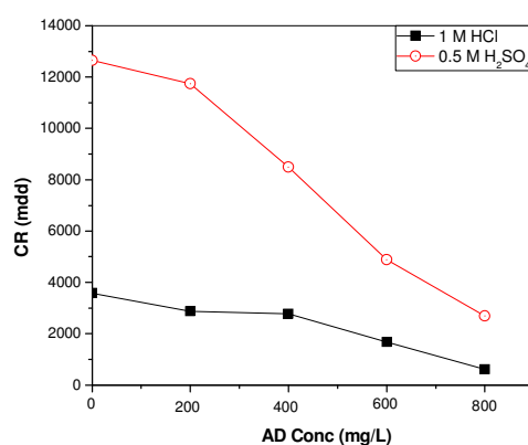
Figure 1. Weight loss of carbon steel 1 M HCl and 0.5 M H 2 SO 4 without and with different concentrations of AD extract.
