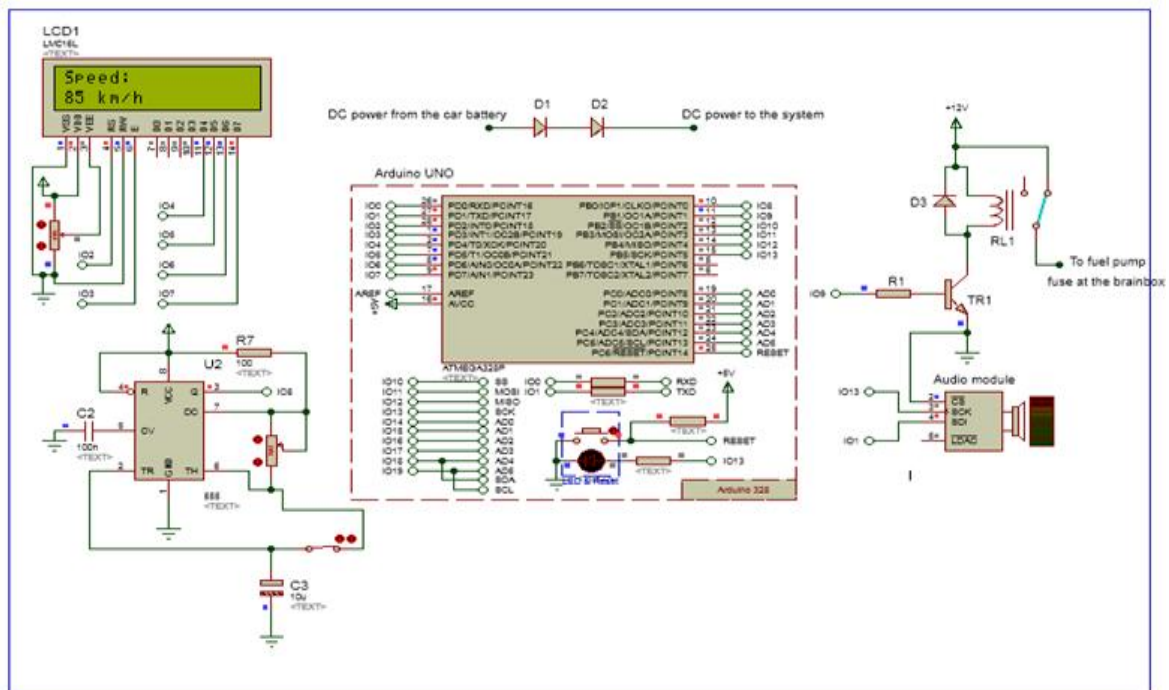
Figure 8. Snapshot of the system when the car was at 85km/hr.
