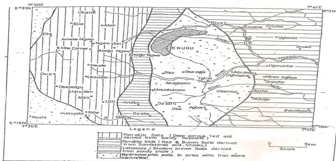
Figure 3. Soil Map of the Study Area
