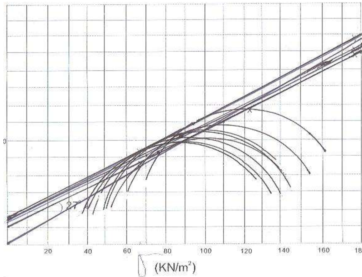
Fig 6: Triaxial Shear Test graph.
