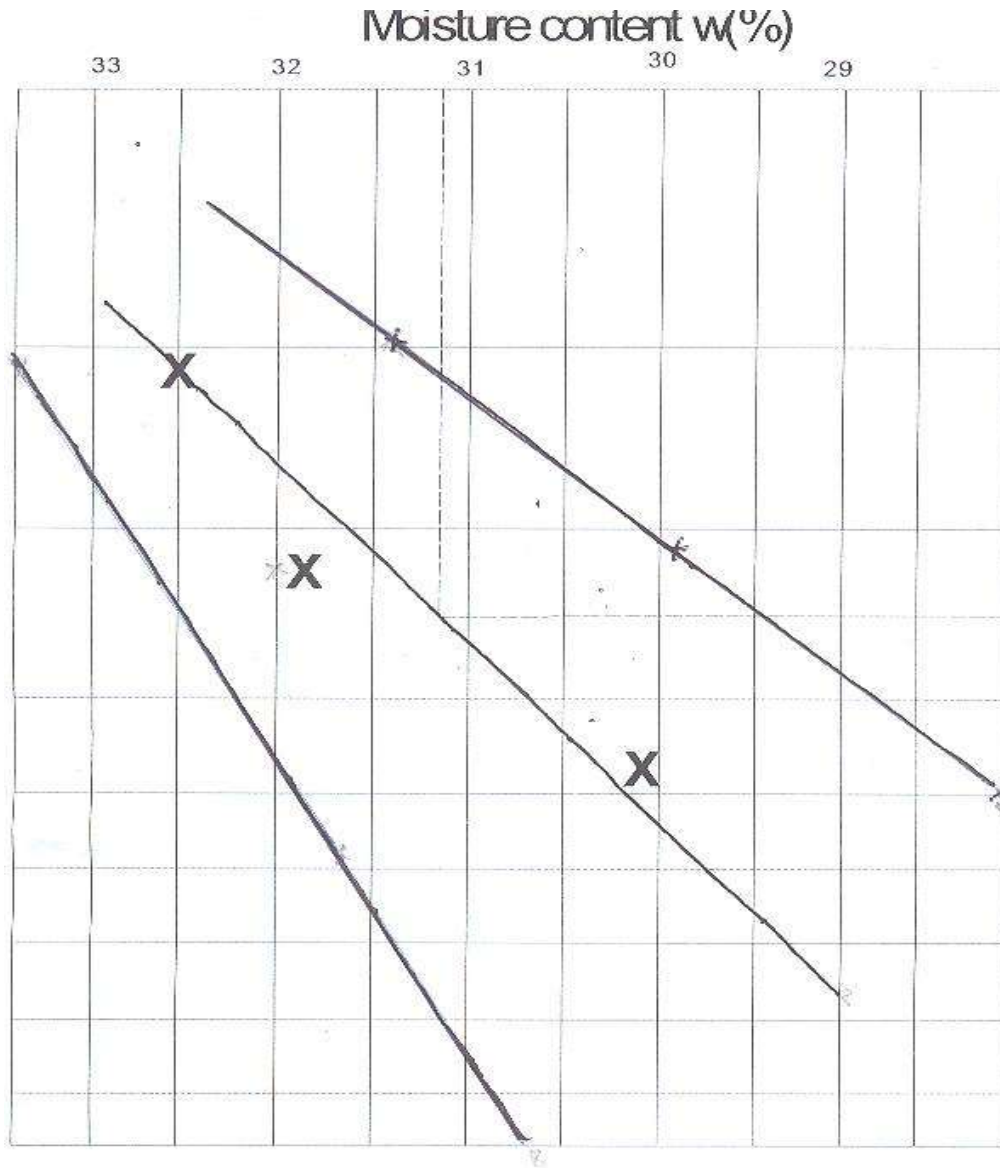
Fig 5: Atterberg Limit Test graph.
