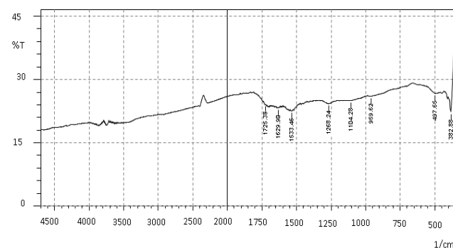
Fig 1: FTIR Analysis of UPPAC.
