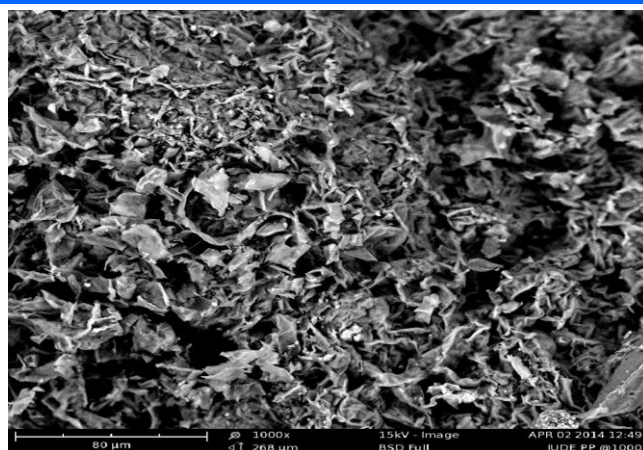
Fig. 5: SEM image of PPAC at 1000x
