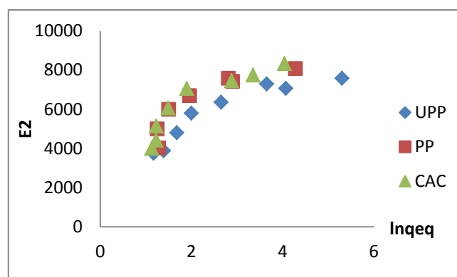
Fig 8 Dubini-Radushkevich Adsorption isotherm of Cu (II) on UPP, PP and CAC at 85°C with pH of 6
