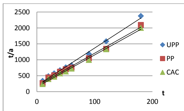
Fig 10 Pseudo-second order plot of the sorption kinetics of Cu(II) of UPP, PP and CAC
