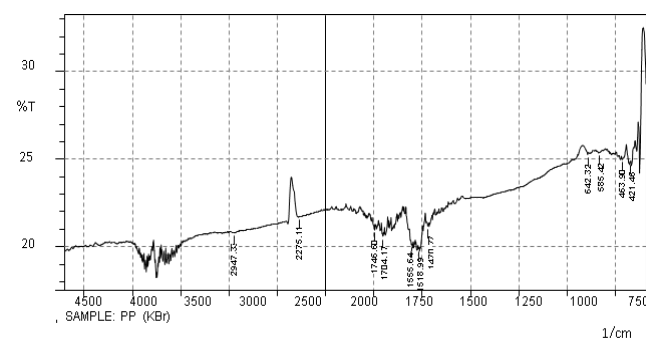
Fig 2 . FTIR Analysis of PPAC
