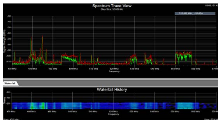
Fig. 1. Spectral analysis plot for frequency span (470 – 570MHz).
