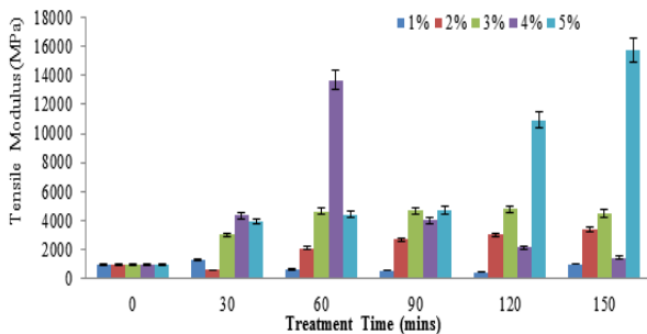
Figure 6: Tensile Modulus of EDTA treated C. populnea fibers
