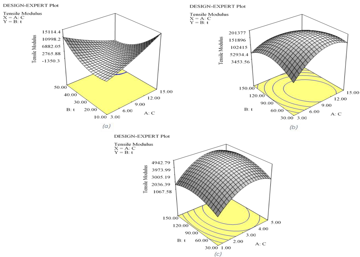
Figure 8: 3-D response surface of tensile modulus of treated C. populnea fibers with (a) NaOH (b) AC (c) EDTA
