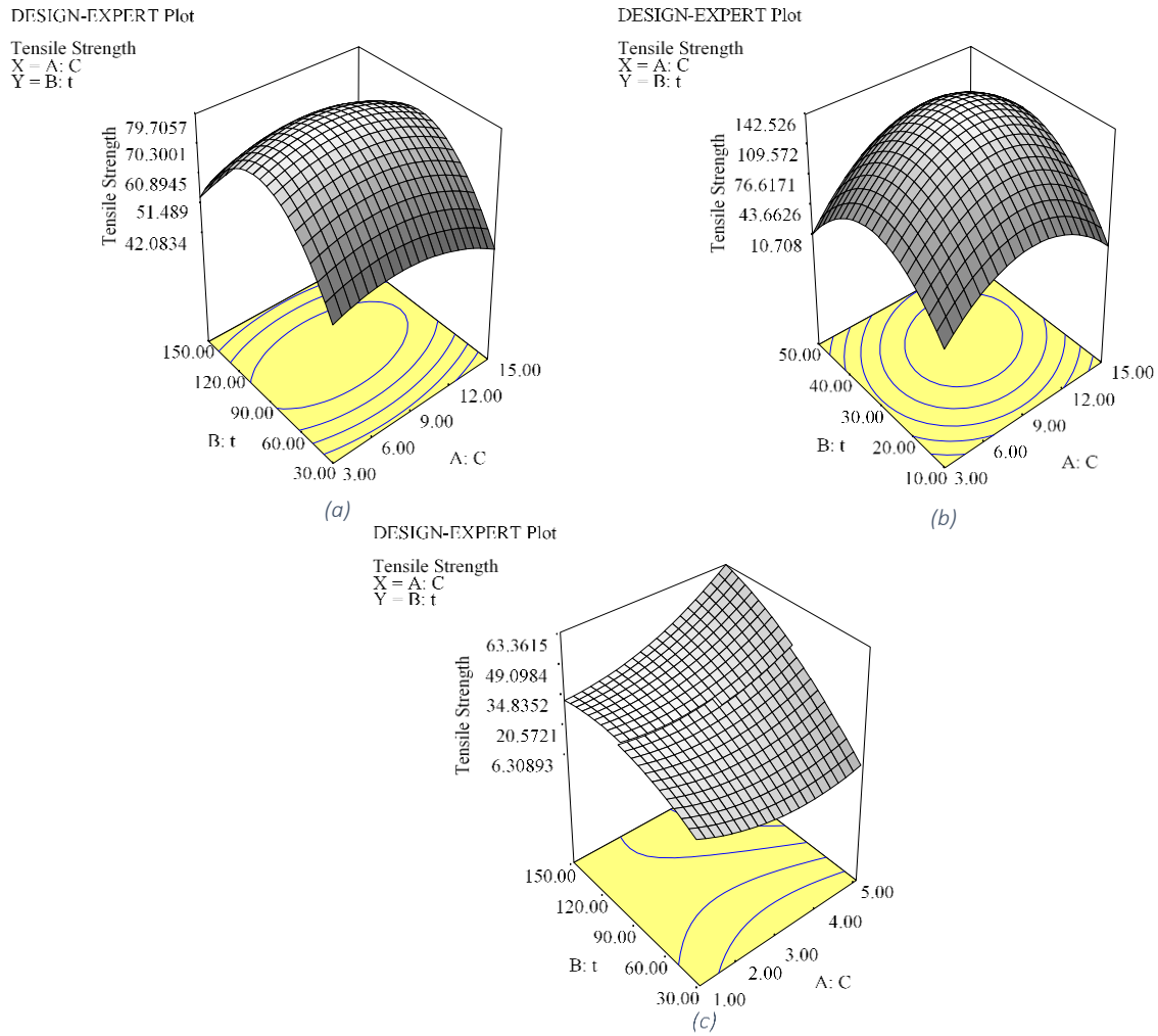
Figure 7: 3-D response surface of tensile strength of treated C. populnea fibers with (a) NaOH (b) AC (c) EDTA
