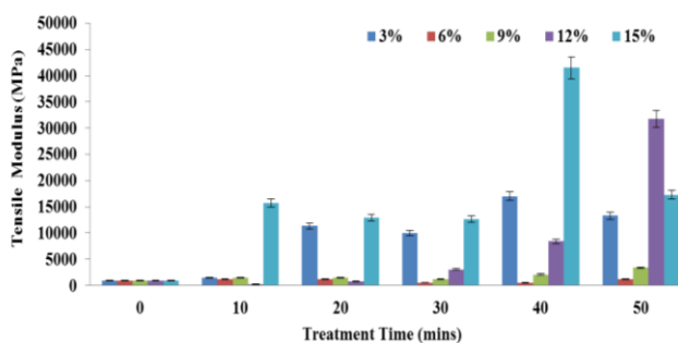
Figure 2: Tensile modulus of NaOH treated C. populnea fibers
