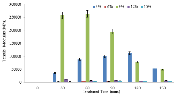
Figure 4: Tensile modulus of AC treated C. populnea fibers
