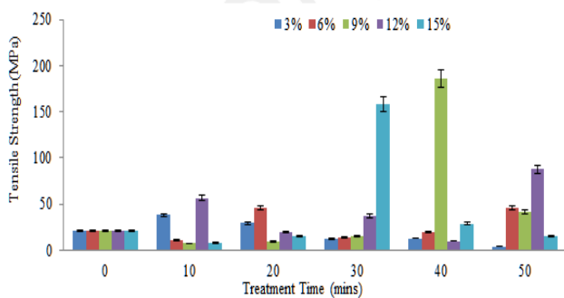
Figure 1: Tensile strength of NaOH treated C. populnea fibers
