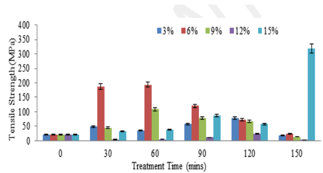
Figure 3: Tensile strength of AC treated C. populnea fibers
