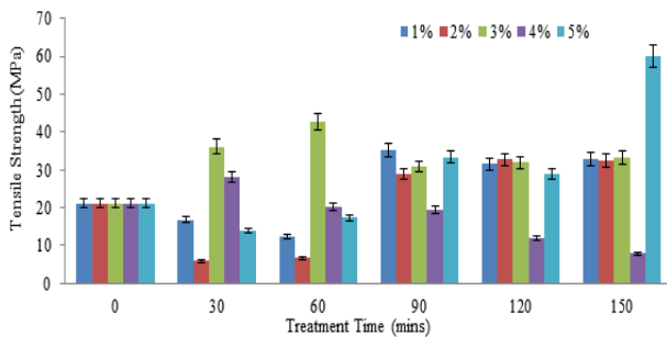
Figure 5: Tensile strength of EDTA treated C. populnea fibers
