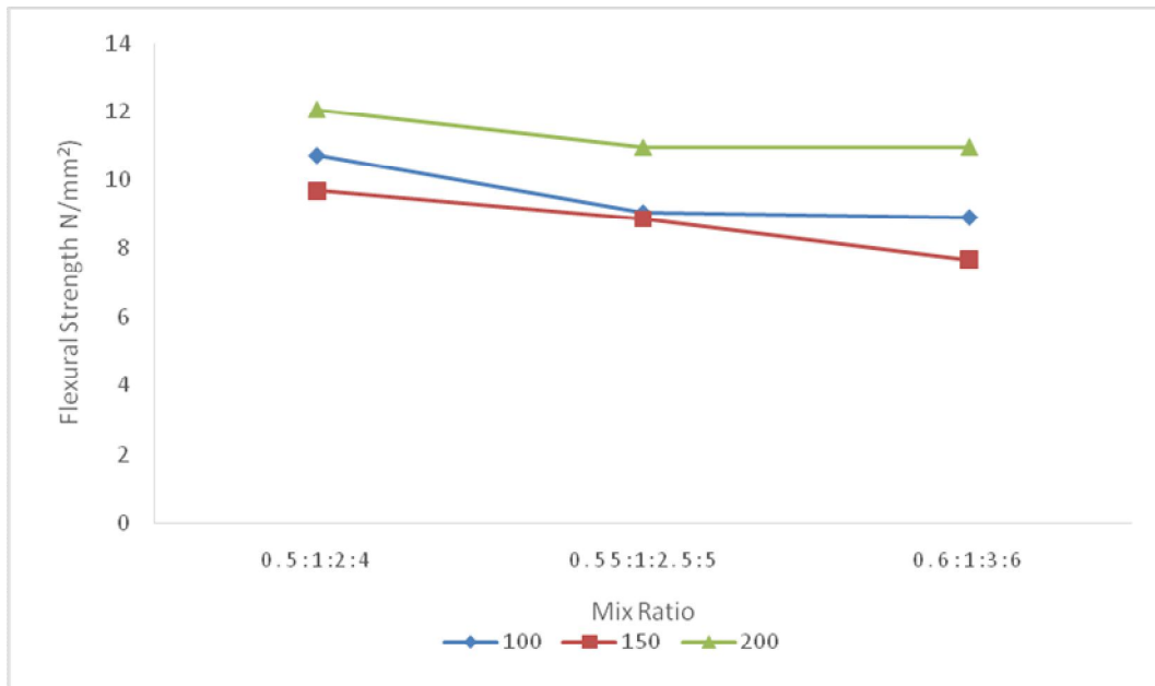
Figure 4.8 Mix ratio against flexural strength of conventional reinforced beam for different spacing
