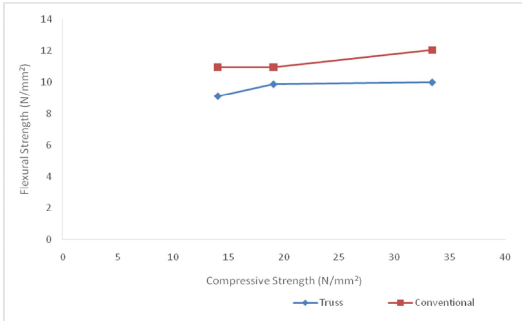
Figure 4.14 Compressive strength against flexural strength of truss and conventional reinforced beam for 200mm spacing
