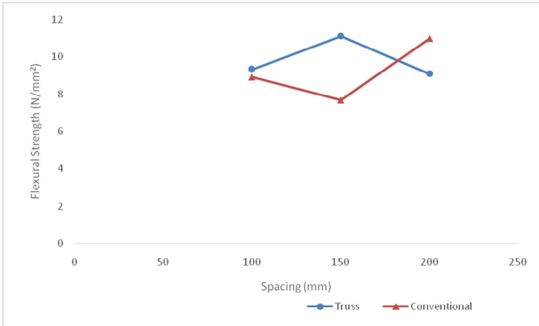
Figure 4.6 Flexural strength against truss and conventional reinforced concrete beam for different spacing for mix ratio 0.6:1:3:6
