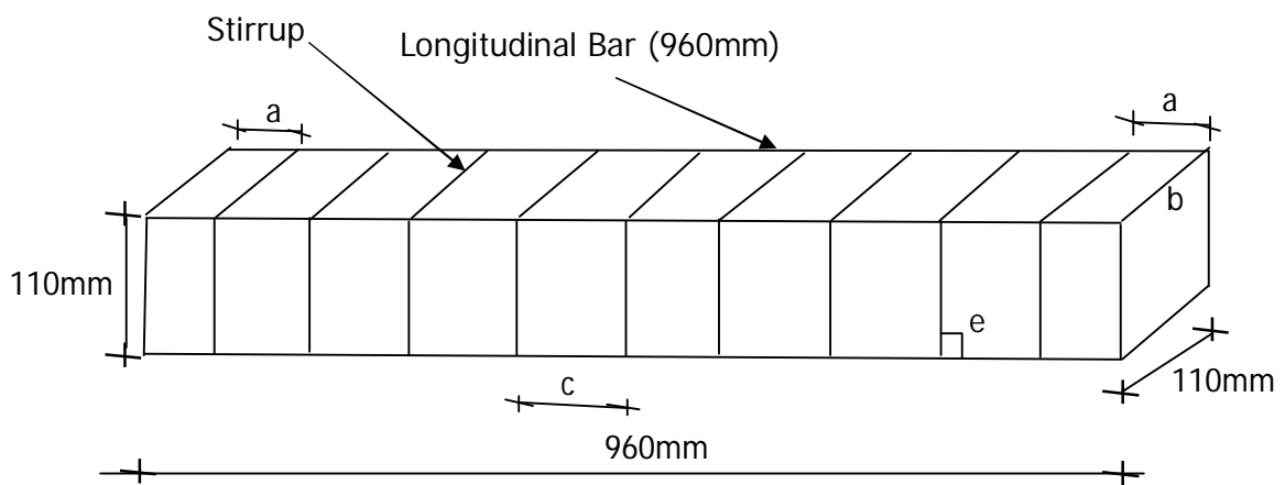
Figure 3.2 Illustration of Conventional Beam Reinforcement
