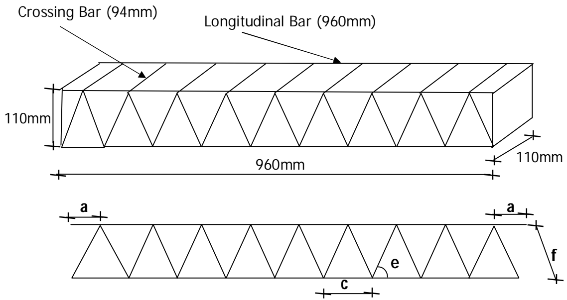
Figure 3.1 Illustration of Truss Reinforcement
