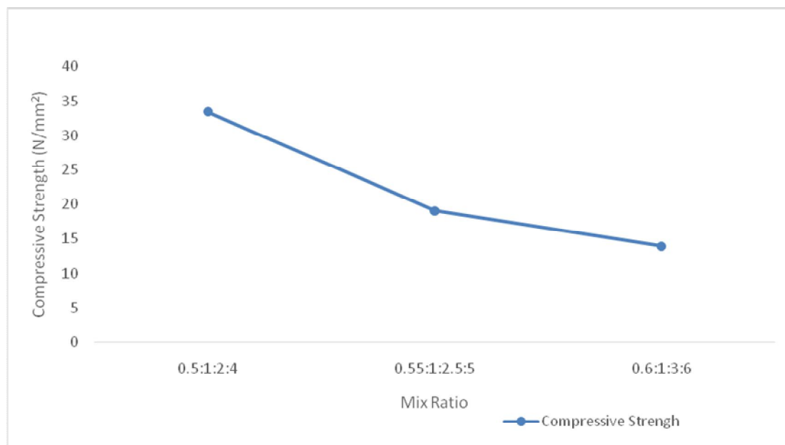
Figure 4.3 Mix Ratio against compressive Strength
