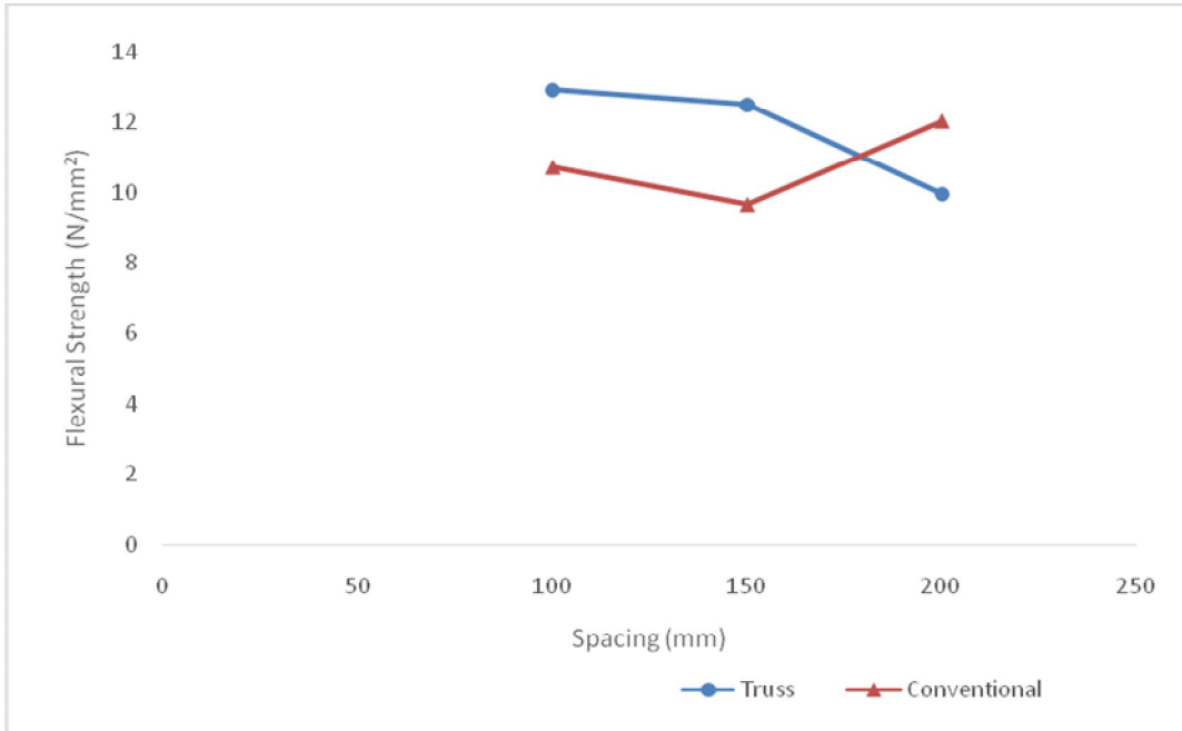
Figure 4.4 Flexural strength against truss and conventional reinforced concrete beam for different spacing for mix ratio 0.5:1:2:4
