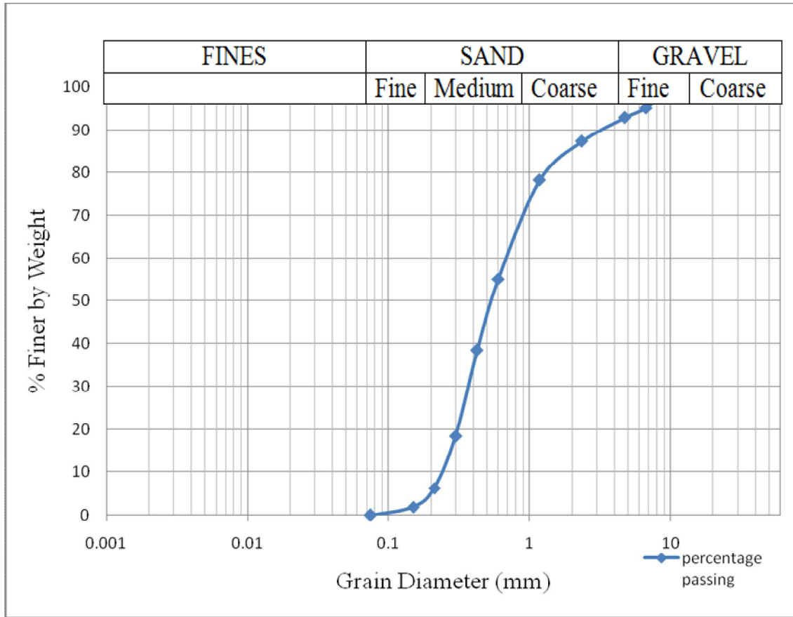
Figure 4.1 Grain Size Distribution of River Sand
