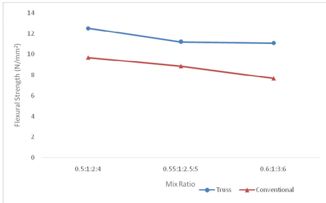
Figure 4.10 Mix ratio against flexural strength of truss and conventional reinforced beam for 150mm spacing
