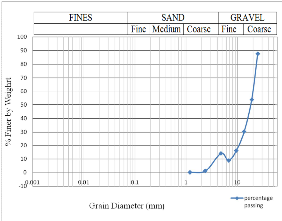
Figure 4.2 Grain Size Distribution of Granite
