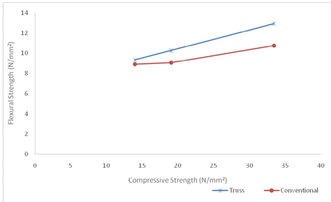
Figure 4.12 Compressive strength against flexural strength of truss and conventional reinforced beam for 100mm spacing
