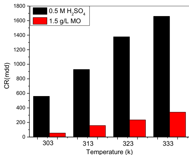
Fig. 2 Effect of temperature during the corrosion of mild steel in 0.5 M H 2 SO 4 in the absence and containing 1.5 g/L MO leaf extract.
