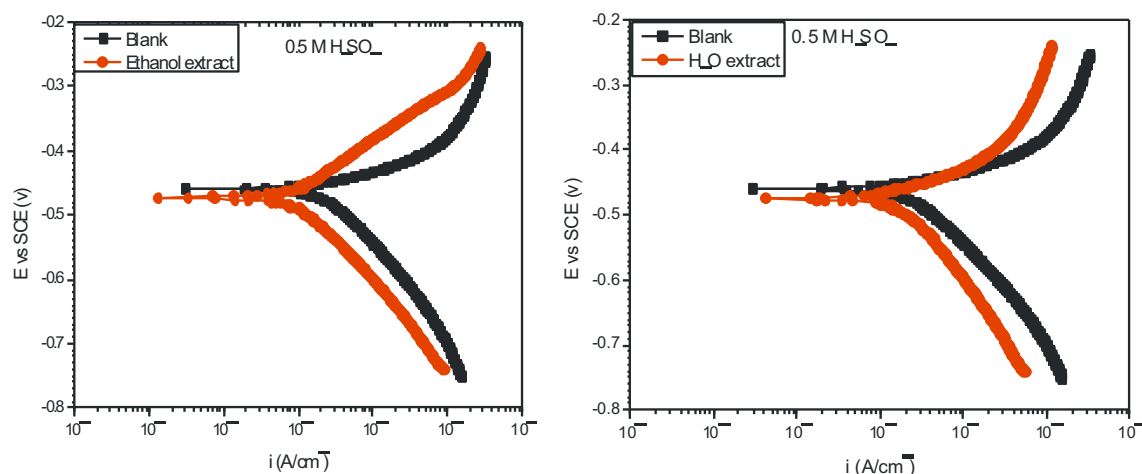
Fig. 4 Potentiodynamic polarization curves of mild steel in 0.5 M H 2 SO 4 solution without and with 1.5 g/L ethanol extract of M.O at 303 K.
