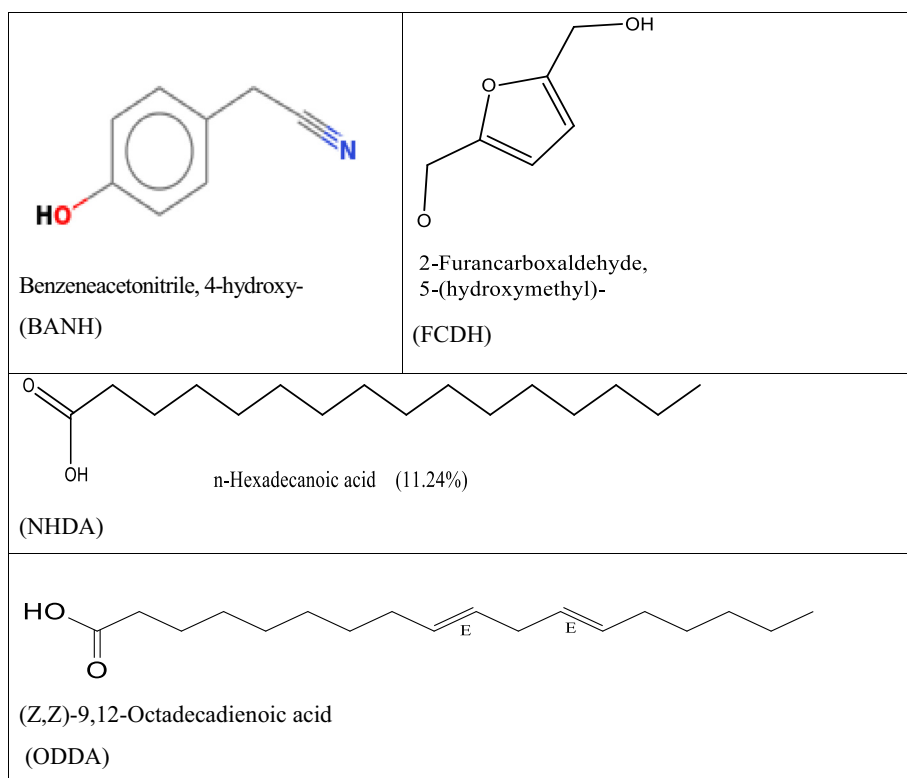
Fig. 11 The molecular structures of plant extract composition, selected for DFT investigation.
