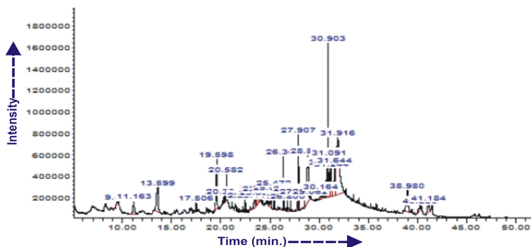
Fig. 10 GC/MS Chromatogram for the ethanol extract of M.O leaves.
