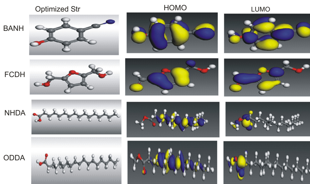
Fig. 12 The optimized geometry structures and the frontier molecular density distribution of the inhibitors (Legend: White = Hydrogen; Grey = Carbon; Blue = Nitrogen; Red = Oxygen).
