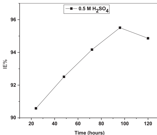
Fig. 1 Effect of time on the inhibition efficiency of MO leaf extract during corrosion of mild steel in 0.5 M H 2 SO 4 at 303 K.
