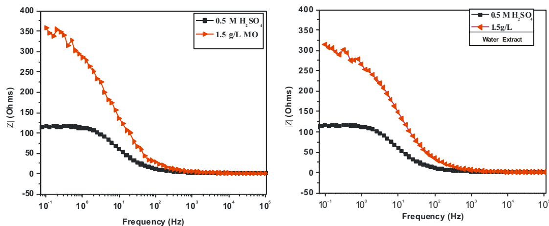
Fig. 6 Bode plot of mild steel in 0.5 M \text{H}_2\text{SO}_4 without and with 1.5 g/L concentrations of MO extract.
