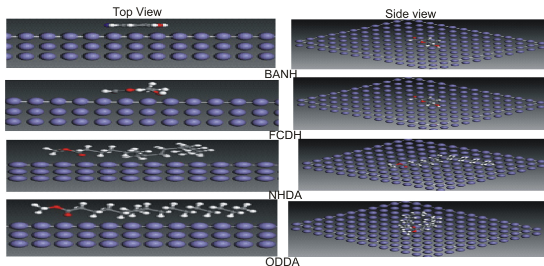
Fig. 13 The equilibrium configuration (top and side views) of studied structures adsorption models on Fe(1 1 0).
