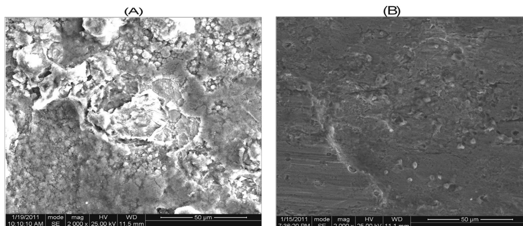
Fig. 8 SEM micrograph of mild steel after immersion in 0.5 M \text{H}_2\text{SO}_4 for 24 h without and with MO extract at 303 K (a and b respectively).
