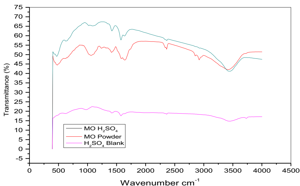
Fig. 9 FTIR spectra of mild steel surface in 0.5 M \text{H}_2\text{SO}_4 at 303 K in the absence and presence of 1.5 g/L of MO extract.
