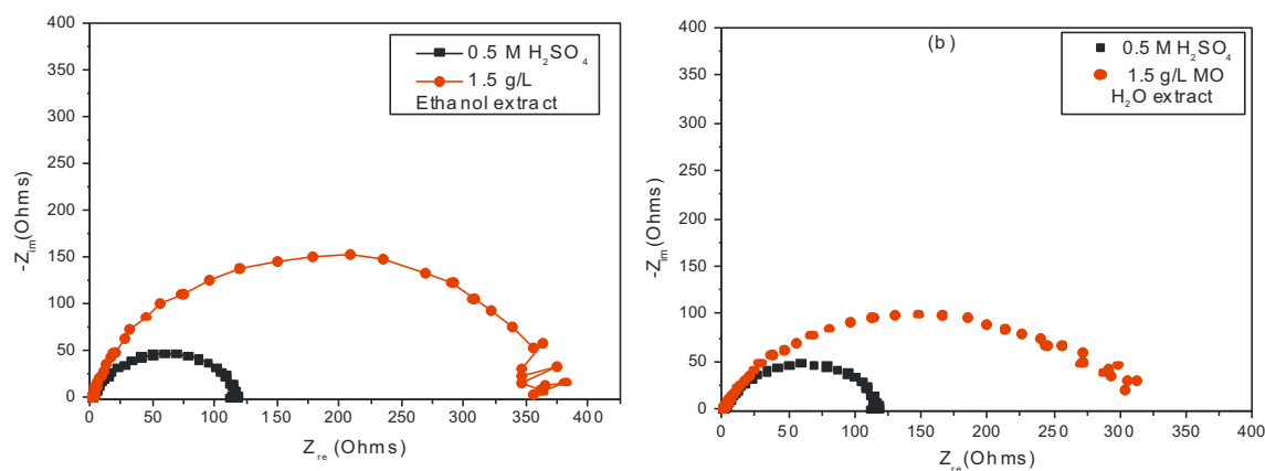
Fig. 5 Nyquist plots for mild steel corrosion in 0.5 M H 2 SO 4 solution at 303 K containing 1.5 g/L concentrations of MO extract from (a) ethanol solvent and (b) from water.
