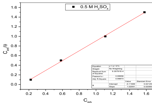
Fig. 3 Langmuir isotherm for adsorption of MO extract on mild steel in 0.5 M H 2 SO 4 at 303 K.
