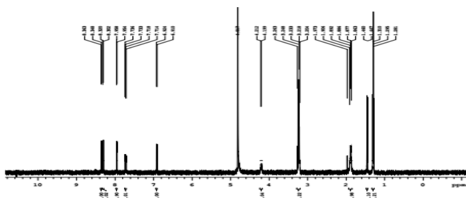
Figure 7: 1 H NMR spectrum of [Sc(CQ) n ]
