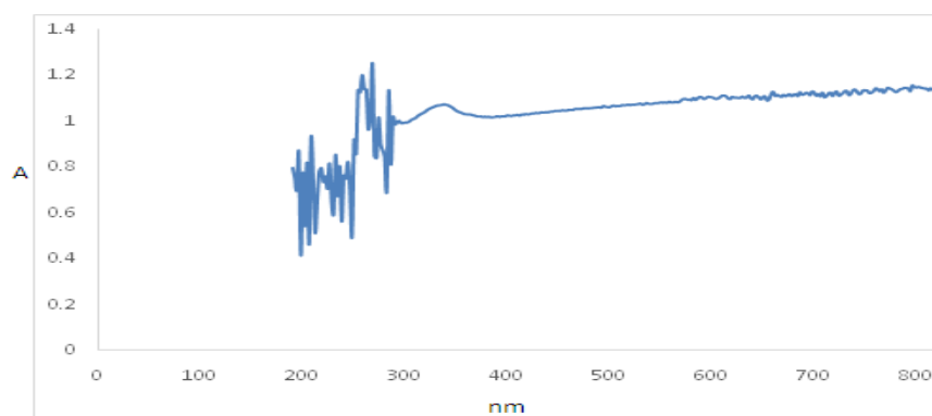
Figure 5: UV spectrum [Sc(CQ)n]
