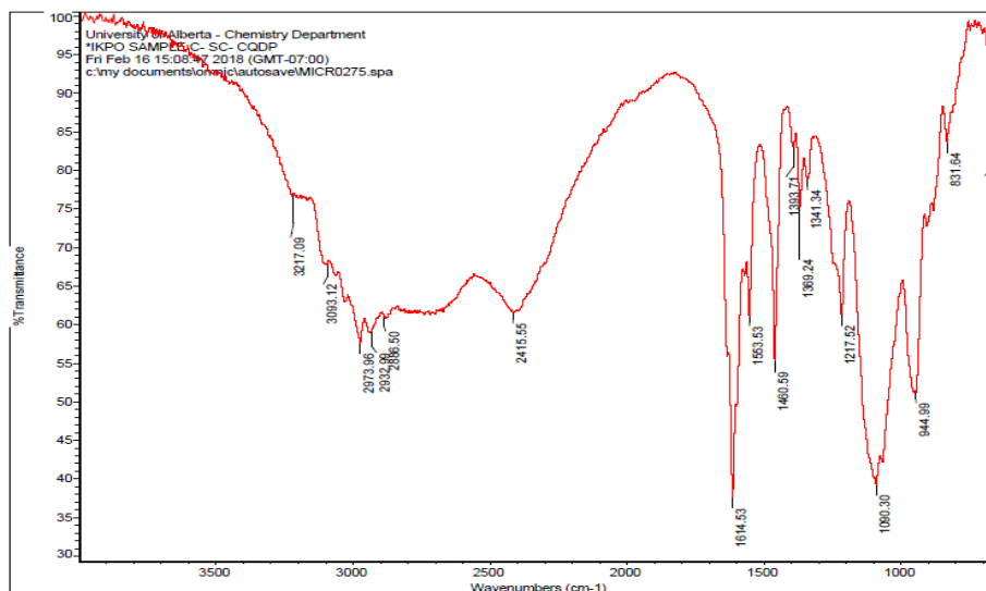
Figure 3: FT-IR spectrum [Sc(CQ)n]
