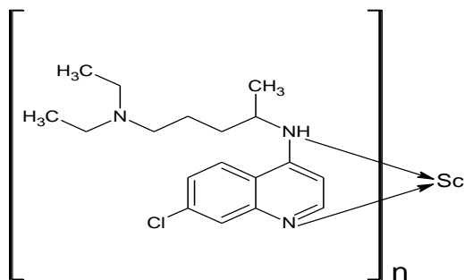
Figure 8. Proposed structure of chloroquine scandium complex, [Sc(CQ)_n]
