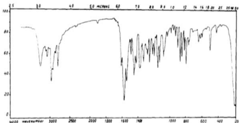
Figure 2: FT-IR spectrum of chloroquine, Source: (Mohammad and Abdullah, 1984).
