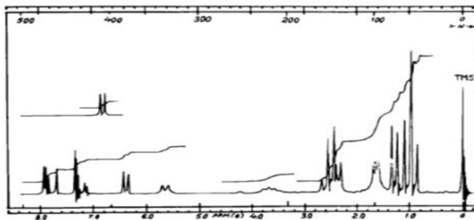
Figure 6: 1 H NMR spectrum of chloroquine, source: (Mohammad and Abdullah, 1984)
