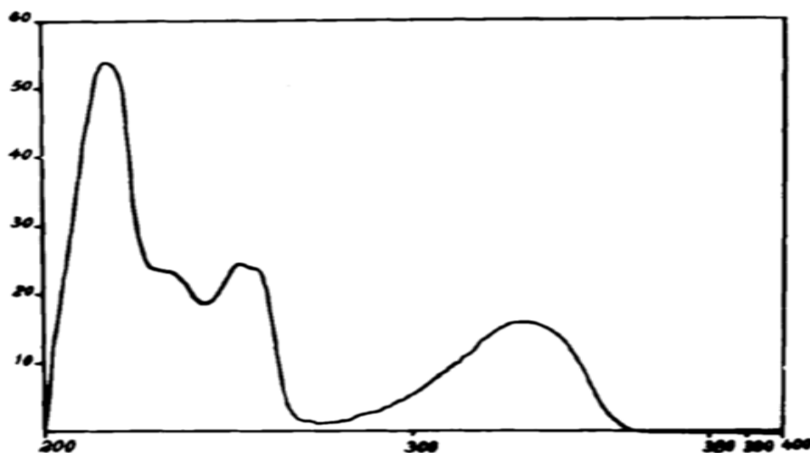
Figure 4: UV spectrum of chloroquine, Source: (Mohammad and Abdullah, 1984)
