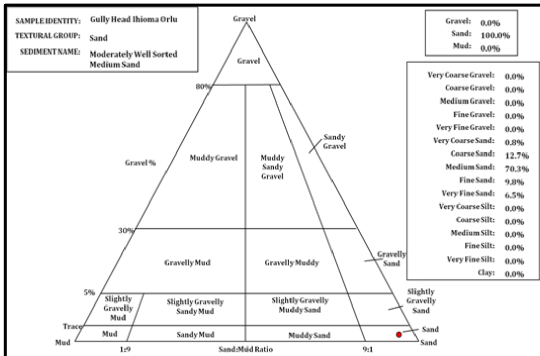
Fig. 4.51: Ternary chart of Ihoma Gully Head grain size distribution
