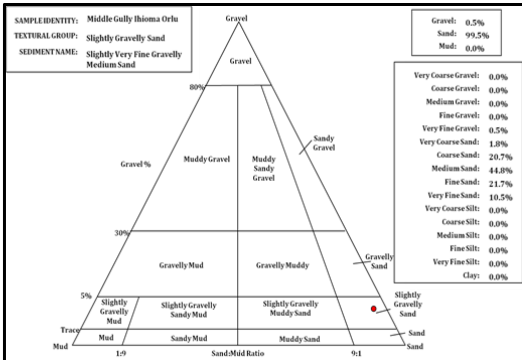
Fig. 4.57: Ternary chart of Middle of Ihioma Gully grain size distribution
