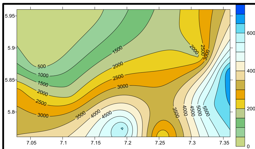
Fig. 4.25: Iso-Resistivity contour at the value AB/2 = 250
