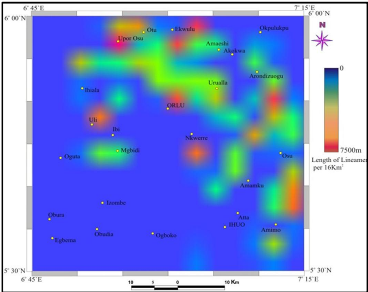
Fig. 4.4: Lineament Density Map of the study area
