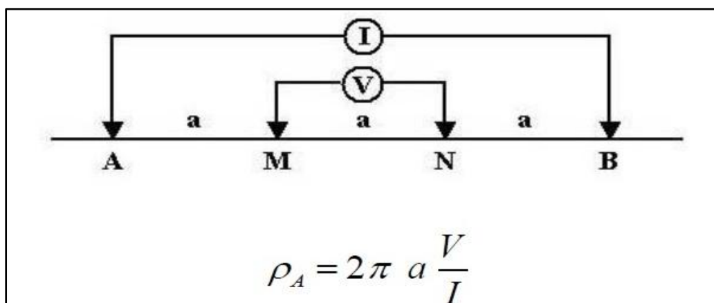
Fig. 2.2: Wenner configuration.
