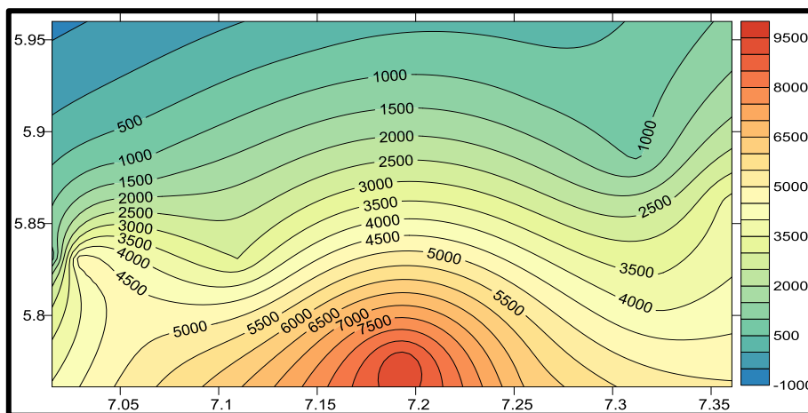
Fig 4.34: The Resistivity contour of the entire fourth (4th) layers – i.e. 4 th from the top most layer
