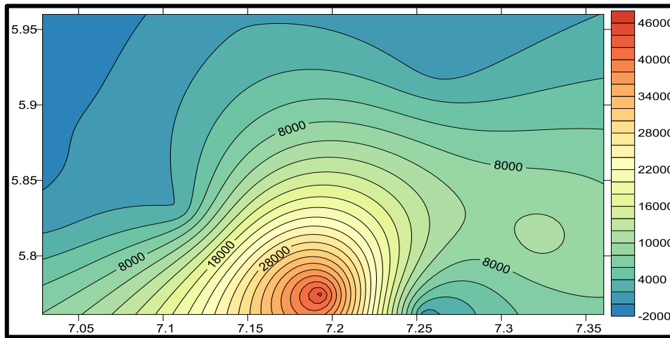
Fig 4.35: The Resistivity contour of the entire fifth (5th) layers – i.e. 5th from the top most layer
