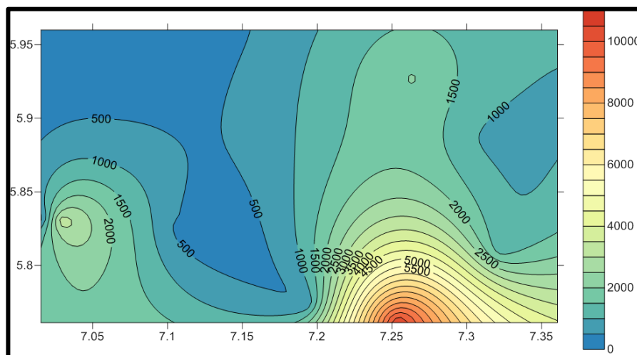
Fig. 4.19: Iso-Resistivity contour at the value AB/2 = 5
