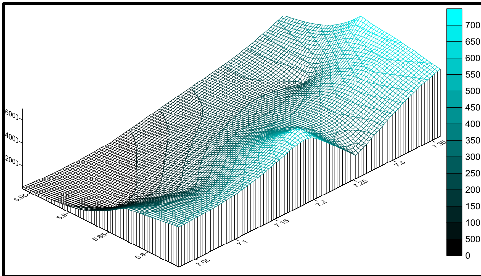
Fig. 4.27: Wired 3D model Iso-Resistivity at the value AB/2 = 250
