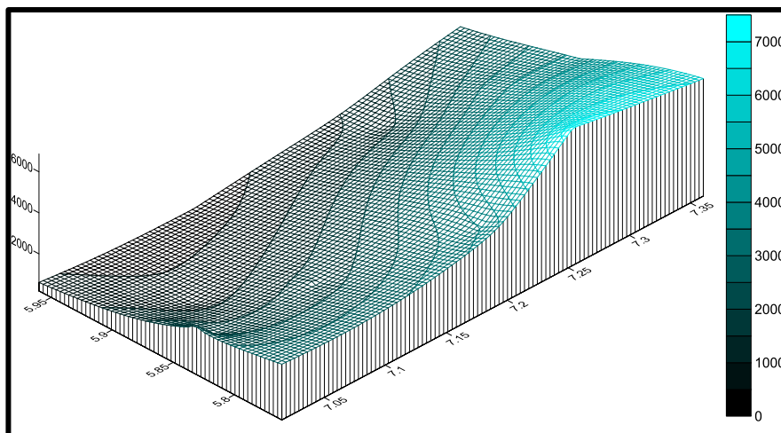
Fig. 4.24: Wired 3D model Iso-Resistivity at the value AB/2 = 125
