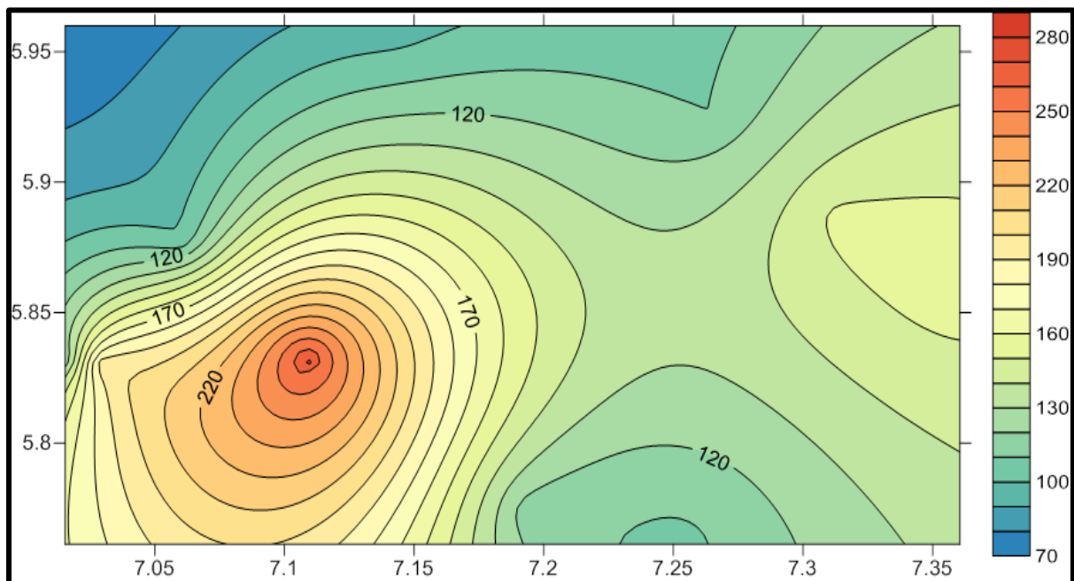
Fig. 4.28: The elevation contour of the study area
