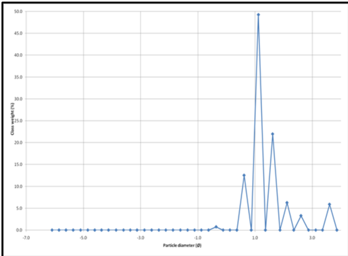
Fig. 4.52: Ihioma Gully Head Grain Size Distribution class of weight graph in phi
