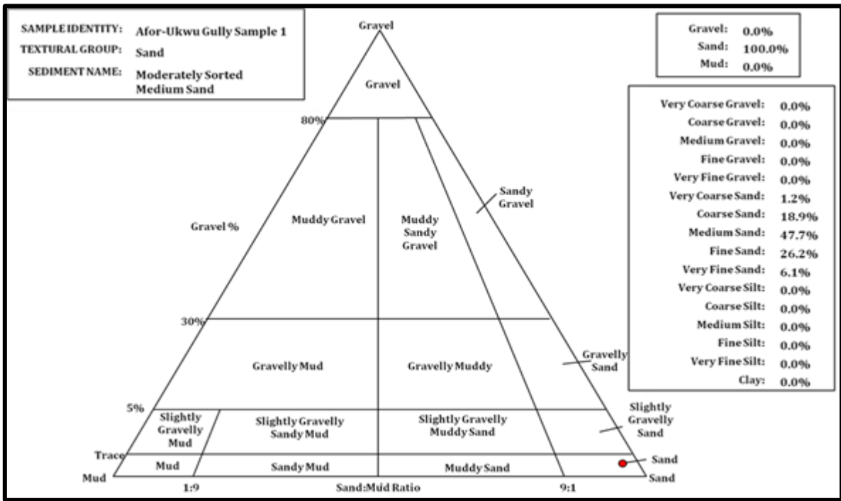
Fig. 4.39: Ternary chart of Afor-Ukwu Gully sample 1 grain size distribution
