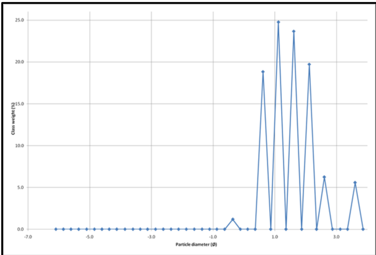
Fig. 4.40: Afor-Ukwu Gully Sample 1 grain size class of weight graph in phi
