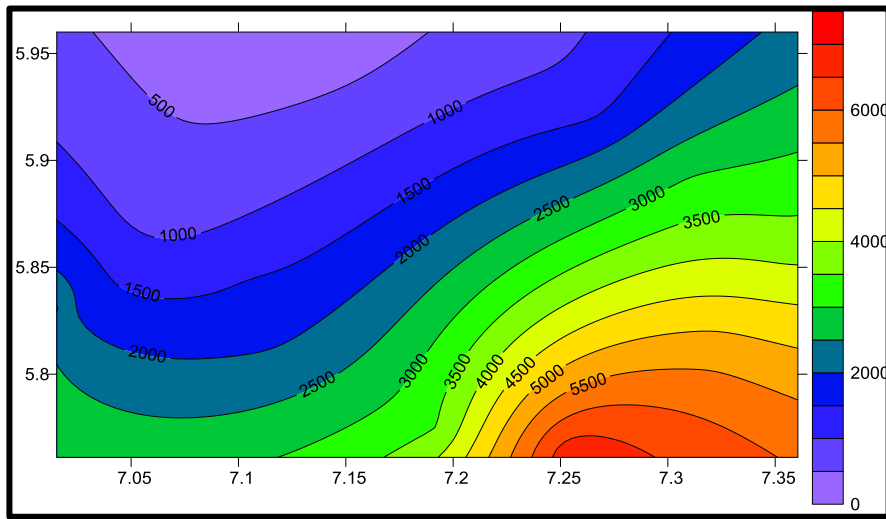
Fig. 4.22: Iso-Resistivity contour at the value AB/2 = 125
