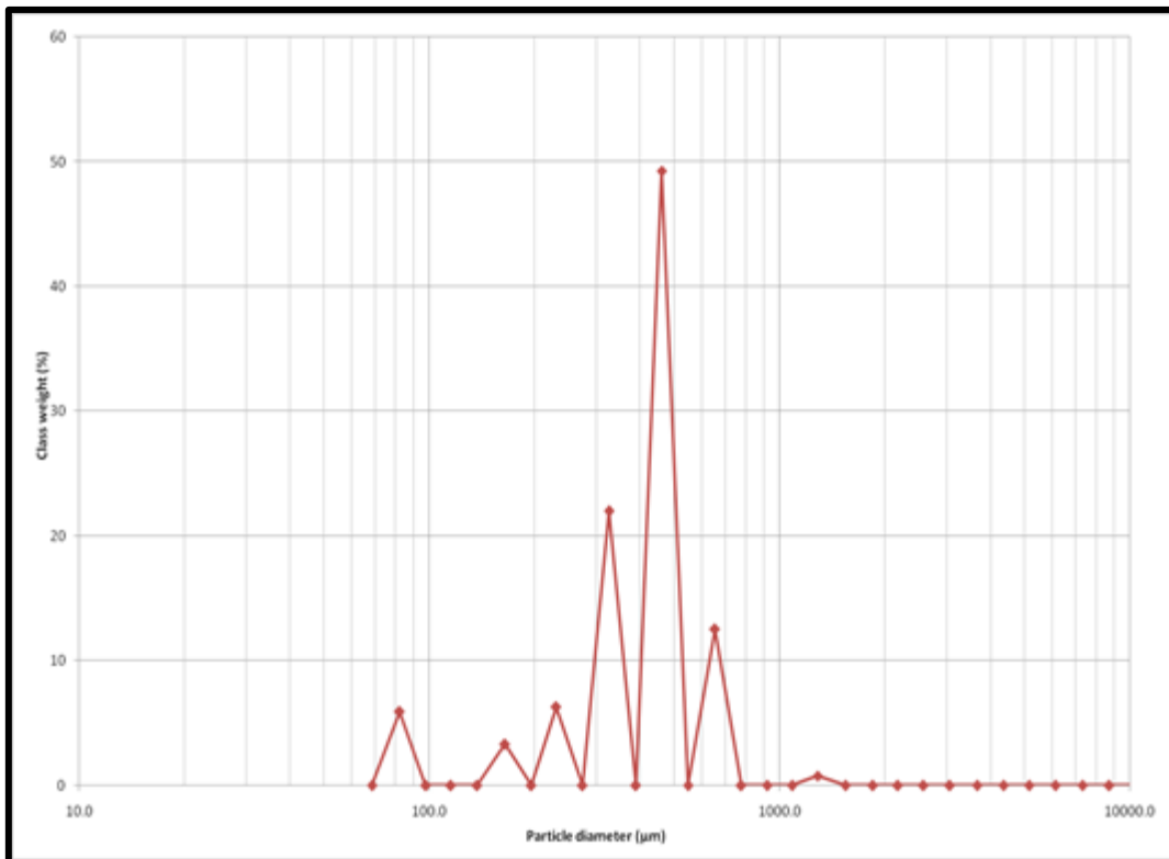
Fig. 4.54: Ihioma Gully Head class of weight graph in microns
