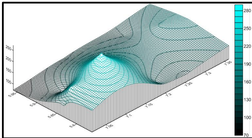
Fig 4.30: Wired 3D Model of the elevation of the study area
