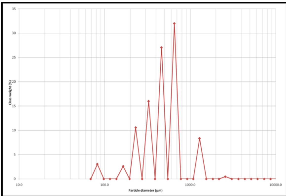
Fig. 4.66: Njaba Gully Sample 1 class of weight graph in microns
