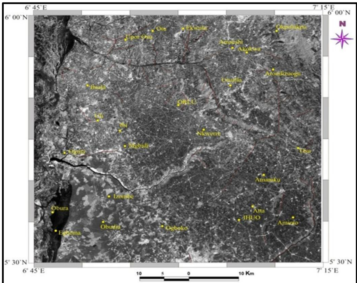
Fig. 4.3: Lineament on Edge Enhanced Band 5 Map of the study area
