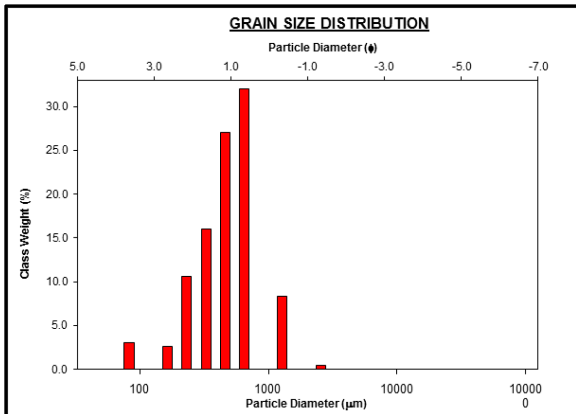
Fig. 4.62: Grain Size class of weight distribution chart of Njaba Gully sample 1.
