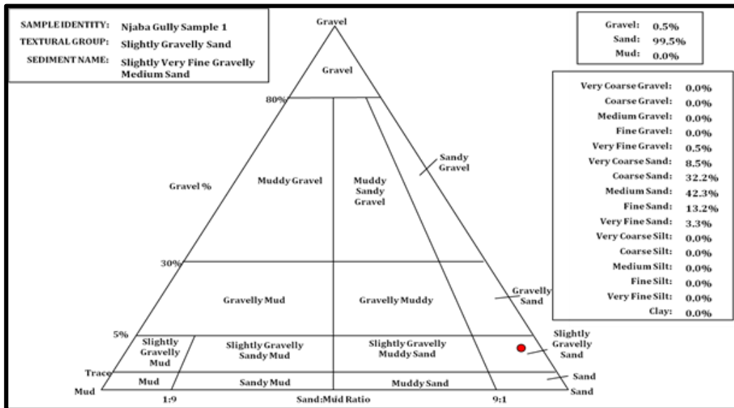
Fig. 4.63: Ternary chart of Njaba Gully sample 1 grain size distribution
