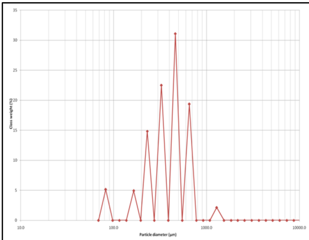
Fig. 4.48: Afor-Ukwu Gully Sample 2 class of weight graph in microns
