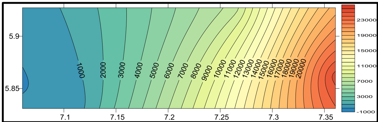
Fig 4.36: The Resistivity contour of the entire fifth (6th) layers – i.e. 6th from the top most layer
