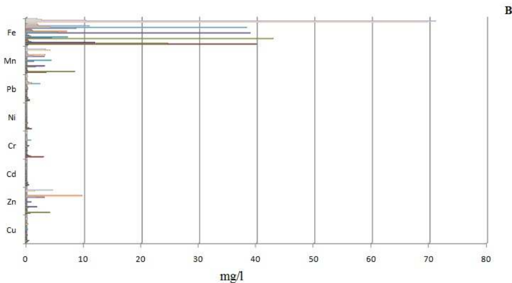
Plot of concentrations of the metals at their respective sampling points
