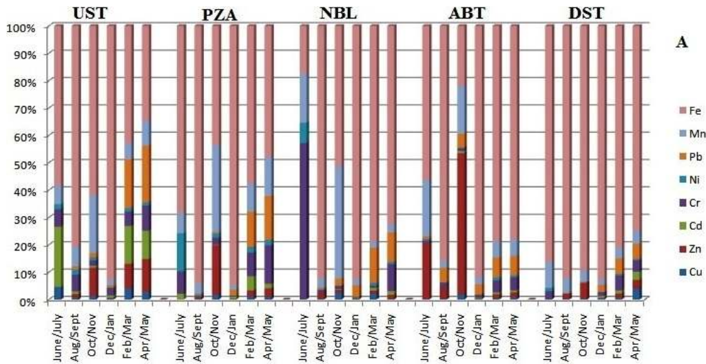
Percentage plot of all the heavy metals showing their proportions at the five sampling point respectively
