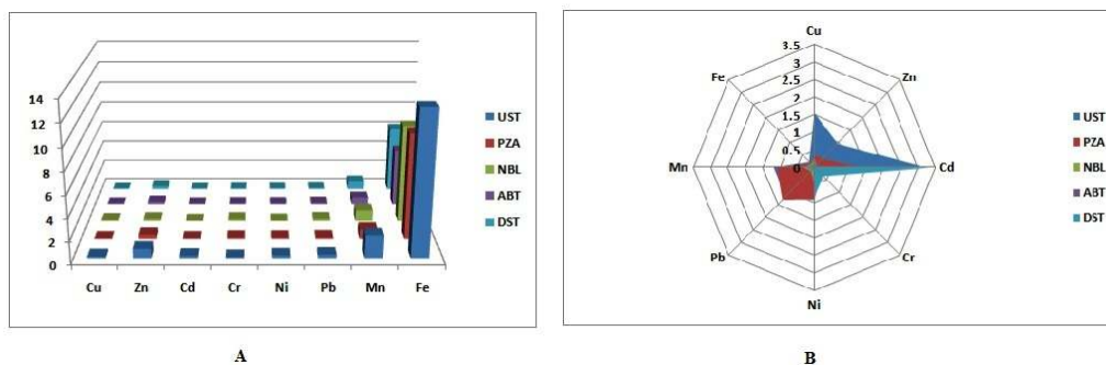
Fig. 2. (A) The average mean values of all sampling points. (B) The bio-concentration factor shown in radar plot
