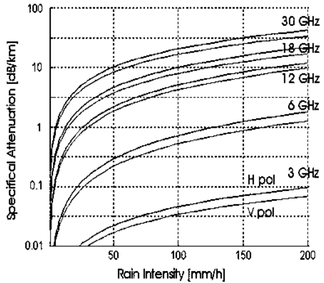
Figure 2. Rain attenuation vs frequency [24]
