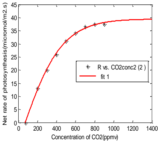
Fig 3a: Net rate of photosynthesis versus concentration of CO 2 absorbed
