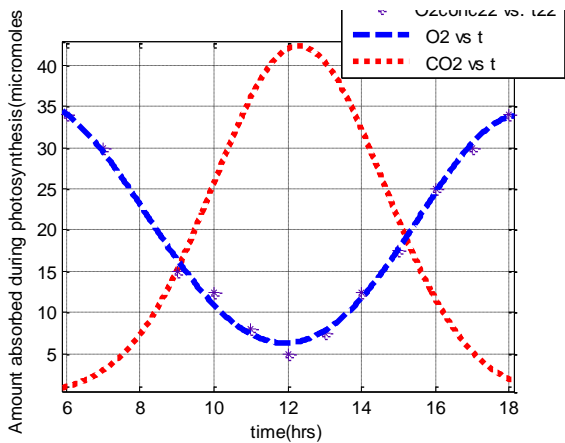
Fig 2: Amount of CO 2 and O 2 absorbed during photosynthesis in a day
