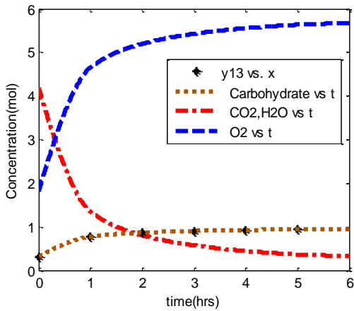
Fig 1: Concentration of CO 2 , H 2 O, O 2 and carbohydrate versus time during daily photosynthesis in the back of a leaf
