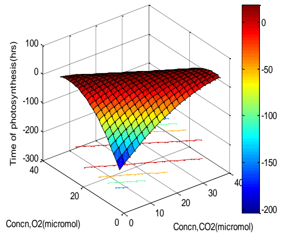
Fig 4: 3-D surface response plot of time of photosynthesis versus Concentrations of CO 2 and O 2 (absorbed by the leaf)
