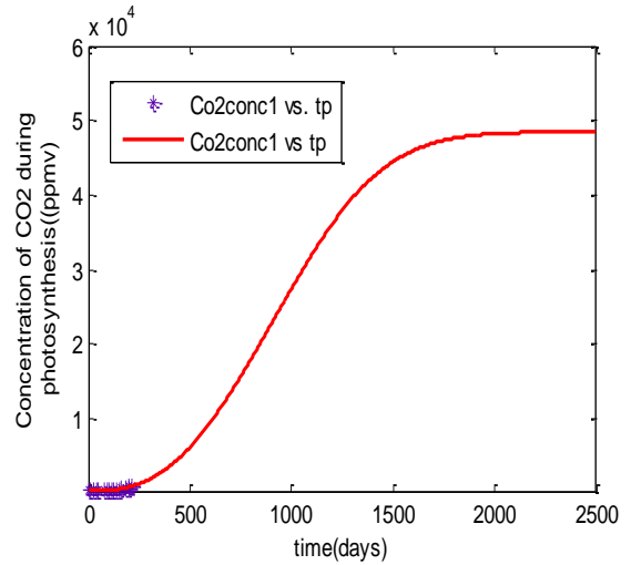
Fig 3b: Concentration of CO 2 during photosynthesis versus time
