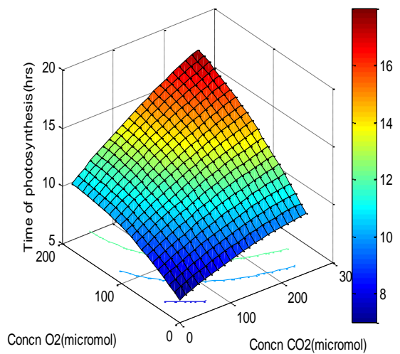
Fig 5: 3-D surface response plot of time of photosynthesis versus Concentrations of CO 2 (taken in) and O 2 (given out) in the reaction
