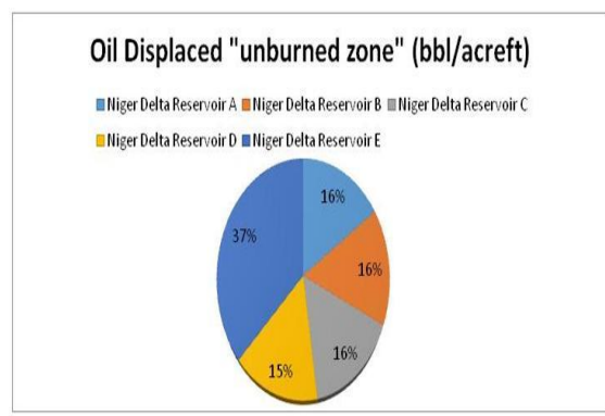
Figure 4: Pie charts showing percentage details of oil displacement from the unburned zones for the five Niger Delta reservoirs considered using the ISC model
