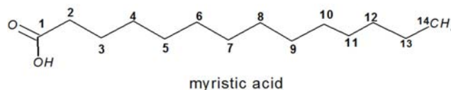
Figure 1a. Structure of Myristic acid.
